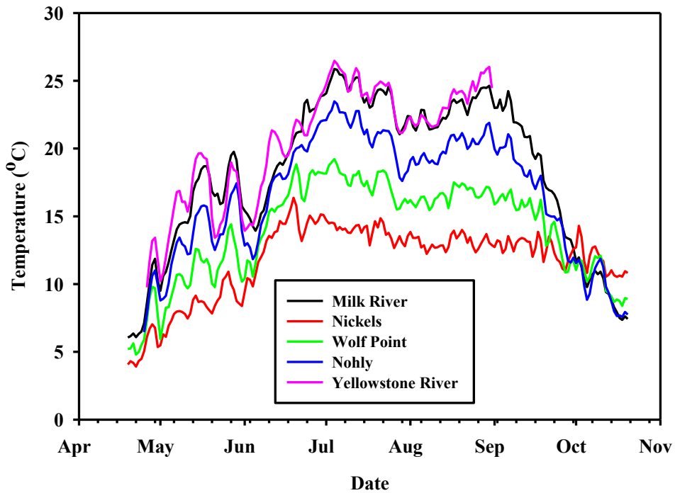
Figure 3. Temperature ( ^{\circ}\text{C} ) at Nickels, Wolf Point and Nohly in the Missouri River, Milk River and Yellowstone River during 2013.
