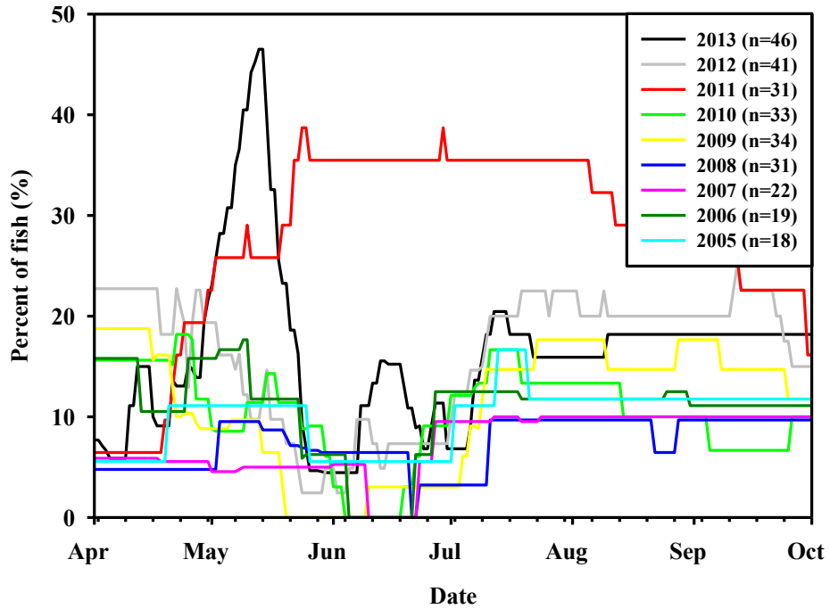
Figure 4. Percentage (%) of telemetered adult pallid sturgeon located in the Missouri River above the confluence of the Yellowstone River by date from 2005 – 2013. N = number of implanted individuals.
