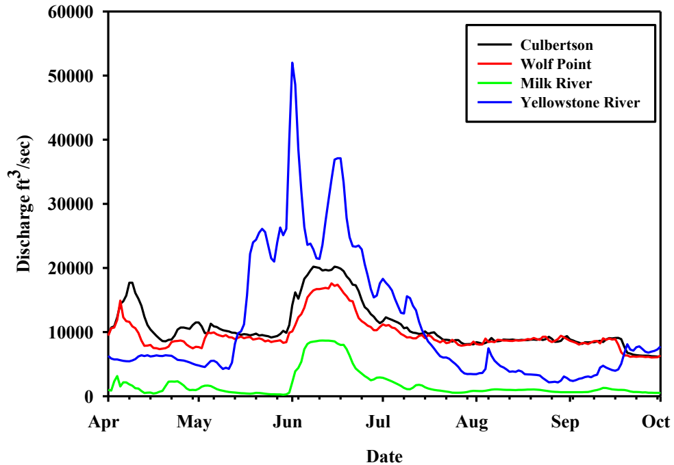
Figure 2. Mean daily discharge ( \text{ft}^3/\text{s} ) in the Missouri River at Culbertson, Montana (gage 06185500), Missouri River at Wolf Point, Montana (gage 06177000), in the Milk River at Nashua, Montana (gage 06174500) and in the Yellowstone River at Sidney, Montana (gage 06329500) during 2013.
