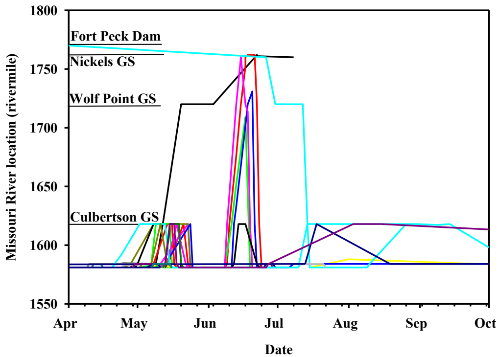
Figure 5. Locations (river mile) of 29 different telemetered pallid sturgeon that used the Missouri River ATC in 2013. River mile 1581 is the confluence of the Yellowstone River, RM 1762 is the Milk River confluence, and RM 1770 is Fort Peck Dam.
